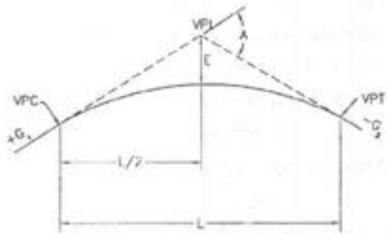
Figure 5: Summit Curve
