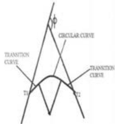
Figure 12: Transition Curve
